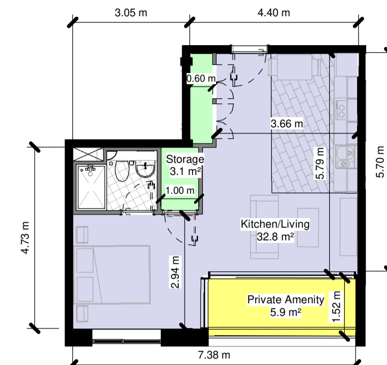
Studio - Type S1.2 1 : 100
