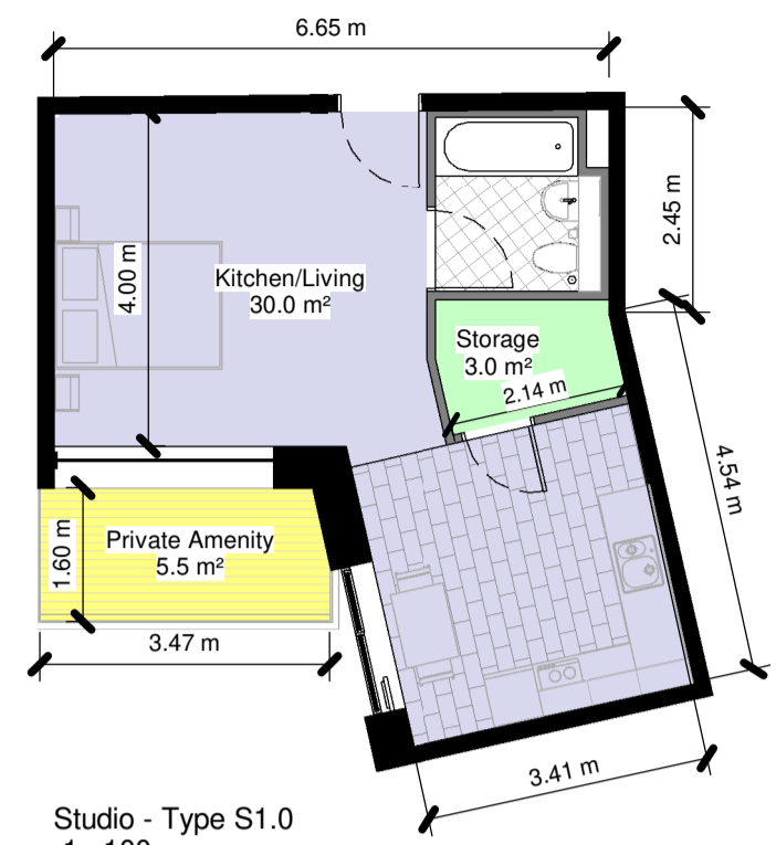
Studio - Type S1.0 1 : 100
