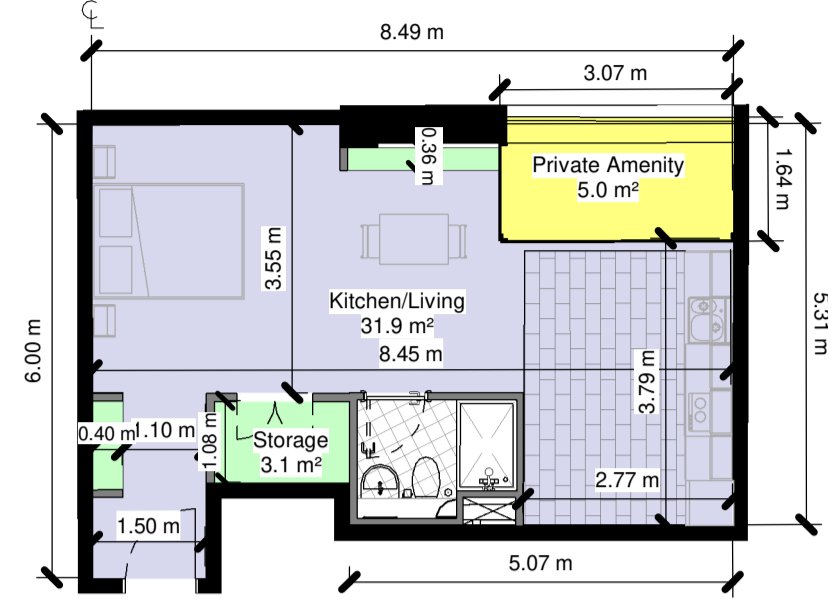
Studio - Type S1.1 1 : 100
